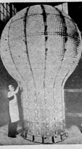
Shown after its recent completion at Corning, N. Y., is the giant electric light bulb which will surmount the $100,000 memorial tower to Thomas Alva Edison at Menlo Park, N. J., where Edison invented the first incandescent electric light. The bulb, 14 feet high, contains 566 electric lights with a 24-inch reflector to be utilized as an airplane beacon.
