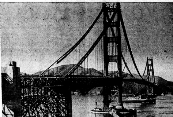
Heralding the approaching completion of the Golden Gate bridge, world's longest single span, the work of stripping away the catwalk construction on the west cable was undertaken. This photograph, taken from the San Francisco side, shows a portion of the catwalk that had already been removed.
