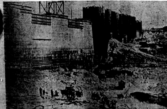
The foundations of the Grand Coulee dam on the Columbia river which will stretch 4,300 feet from cliff to cliff and rise 350 feet in height, at which an army of men are now at work.
