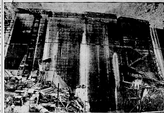
When this photograph of the upstream face of Boulder dam was taken the other day the millilith cubic yard of concrete had just been poured, and the giant structure was almost one-third completed. The view is from the collieries.
