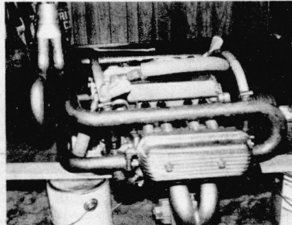
The water-cooled engine, made especially for the Scorpion was assembled in Kenneth's garage.
