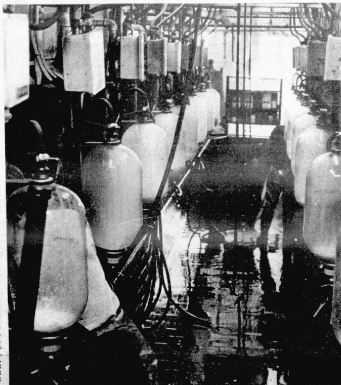
This double 8 herringbone parlor at Dressel Dairy, Inc., was one of the first two in the state. It can handle 85 cows per
