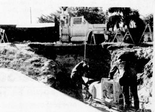
A NIPPY BREEZE whipped off Lake Verona as Star Tell, Inc. workmen bored the last 24 inch pipe under Main St. last week. The pipe will carry a gravity line and a force main sewer pipe from a lift station across
