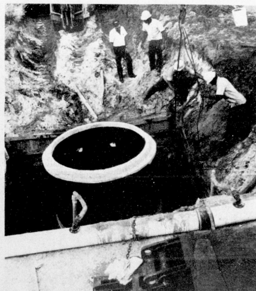
WITH TWO SECTIONS OF six foot inside diameter precast concrete pipe in place 17 feet deep workers prepare to attach cables to the cofferdam to remove it. The top section of concrete pipe weighs about 8000 pounds while the bottom section weighs
