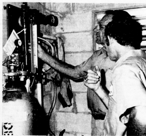
CAROL BROOKSVILLE, representing Wallace & Tiernan and Co., manufacturers of chlorinating equipment, discussed with Rainey Prevatt (right) how the quantity or flow of chlorine into the water mains affects the height of the small ball in the glass tube of the rate of flow gauge. Tanks of chlorine set to the left of the control unit. Photo—Miller.
