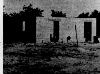
THIS TWO ROOM structure will house the pumping facilities of the new well on W. Bell Street near the airport. The 14 inch well with a 12 inch pump will be geared to inject 1400 to 1800 gallons of water per minute into the city water system. Chlorination equipment will be installed in the second room. (Photo-Miller).
