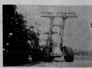
The articulating steering aids greatly in maneuverability of this machine as shown as the loader circles a citrus tree. This too, aids in reducing tree damage to the grove.
