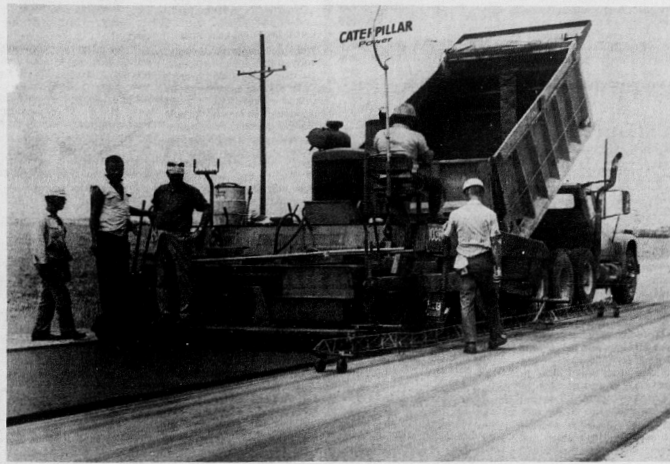
EWELL CONSTRUCTION Company of Lakeland, under contract with the county are resurfacing three miles of city streets, along with county roads. The big Barber-Greene can be seen here laying the hot asphalt on the Bombing Range
