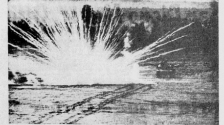
SMOKE SHOOT —Sheridans (above left) of the 3rd Sq. 4th Cav. 8th Inf Div. prepare to move out. Circled are four of the vehicle's eight grenade launchers. Down range a smoke and phosphorus grenade (above right) explodes and the smoke screen makes 14.5-ton vehicle almost invisible in bottom left photo. When clearing the screen the Sheridan is doing fast flip. The demonstration took place on Range 80 at Grafenwoehr.
