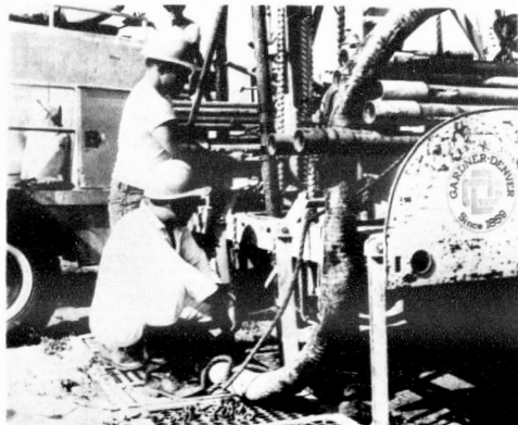
SOIL BORINGS at Lake Anoka were taken last week as Florida Department of Transportation sought to determine the best way to repair the collapsed road bed of US 27. (Photo by L. Miller)
