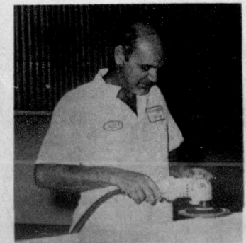
BILL WHITE of Avon Park smooths out rough edges of a boat deck at Critchfield Marine's boat plant. The boats are built from the outside to the inside, beginning with the application of a layer of paint to a re-usable mold. Then the fiberglass strands are laid on the paint, resin and a catalyst are applied, and chopped fiberglass is spread over the surface.
