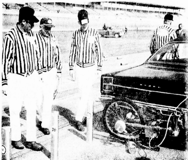
Smashed equipment resulted when this sedan slewed completely around in braking test. Car was moving to left of picture when brakes were suddenly applied.
