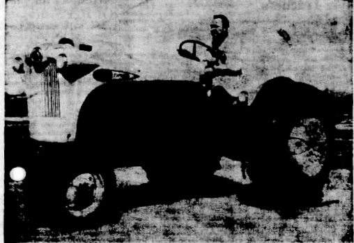
The first known installation of a free piston turbine engine in a tractor is announced by Ford Motor Company's Tractor and Implement Division. Strictly experimental, the Ford Tractor is powered by a single cylinder engine having two free-moving pistons. The pistons produce gas under pressure which drives a turbine, providing smooth power with greatly reduced vibration. The Typo has now utilized about half of the 100 horsepower which the engine is capable of producing.
